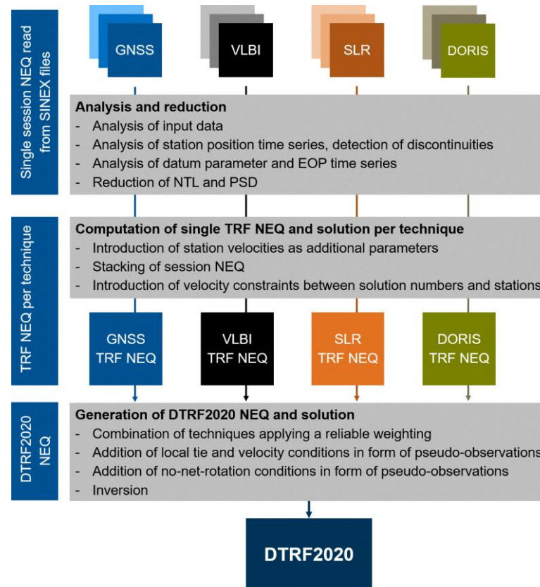
Fig. 1: DTRF2020-u2023 computation strategy.
